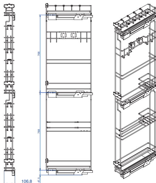
Estraibile laterale portascopa Side pull-out broom holder
